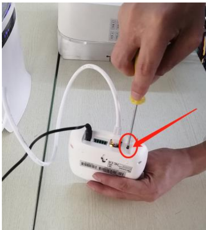
Figure5.bottom button position
