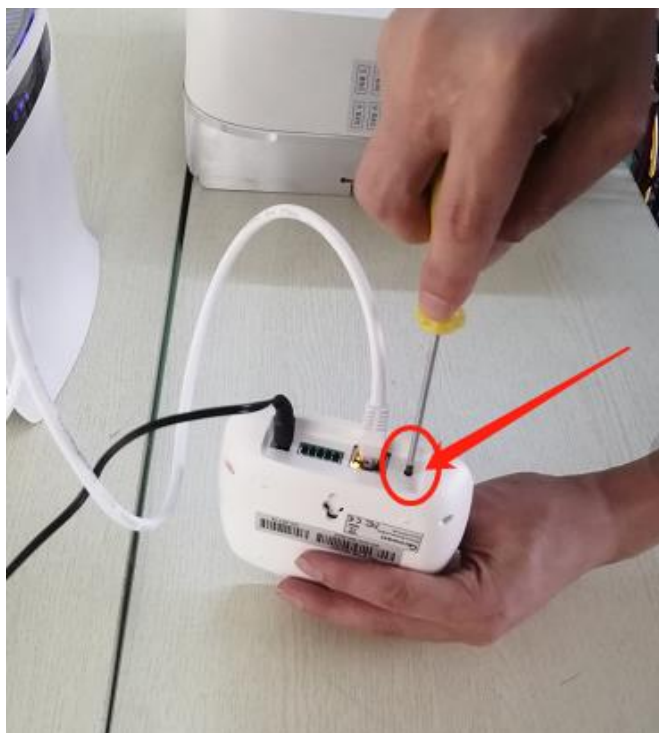
Figure5.bottom button position
